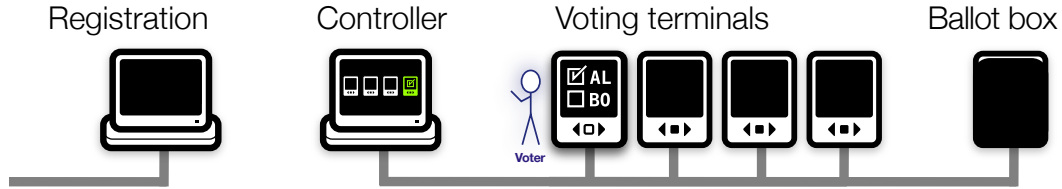
Fig. 1. The design of the STAR-Vote system. The voter registration system (left) is connected to the Internet but not to the internal LAN. Voters move left to right. First, the voter's registration is validated, and a thermal printout indicates the proper ballot style. This moves to the controller, which scans it and issues the voter a PIN, again printed on thermal paper. The voter proceeds to any open voting terminal, enters the PIN, and is given the proper ballot style. The ballot summary is printed, and deposited into the ballot box (right).
